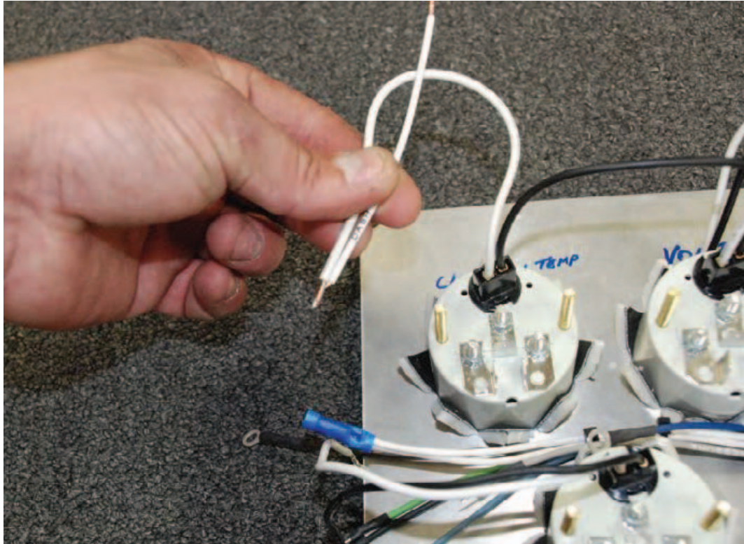
Twist the gauge light power wire from the Oil Temp gauge with one of the small white jumper wires.
