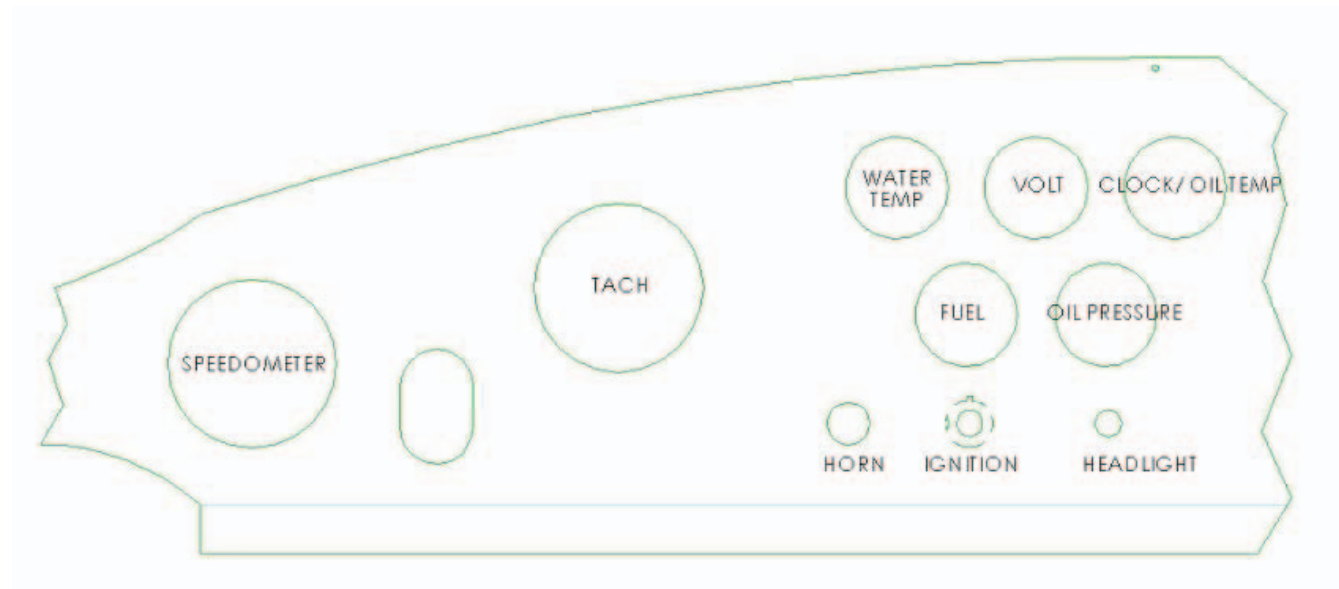
Standard Roadster laser cut gauge layout.
