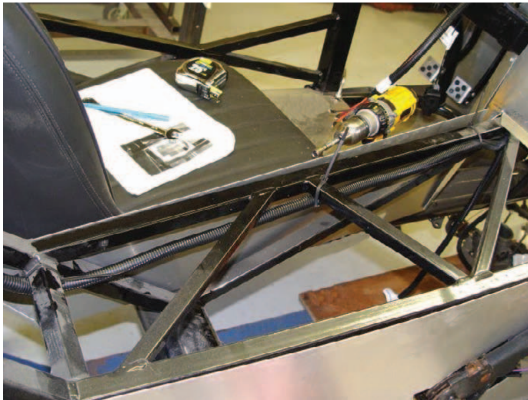
Using zip ties included with the kit to hold the harness in place, run the harness along the driver top transmission tunnel tube and up to the 2"x 3" tube at the back of the cockpit.
