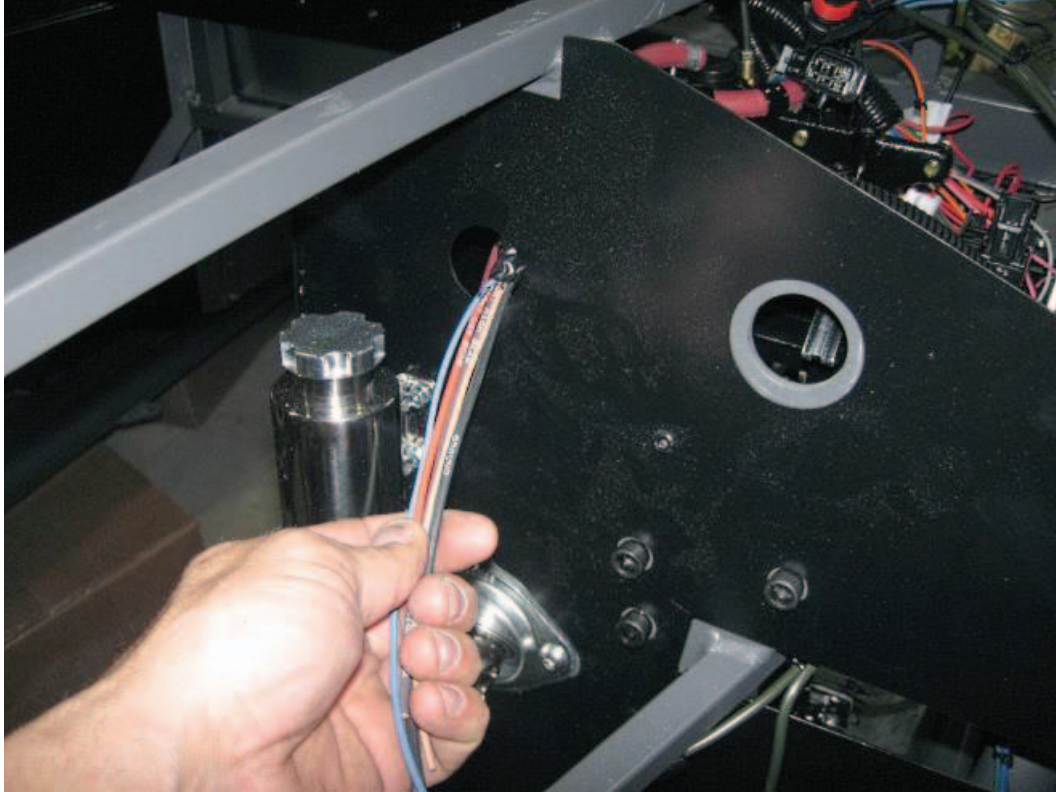
Pull the front harness all the way through the small right hole in the front of the footbox.
