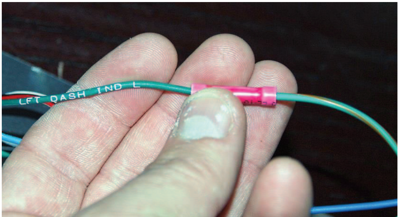
Connect the green left turn indicator wire to the gauge green/yellow wire.
