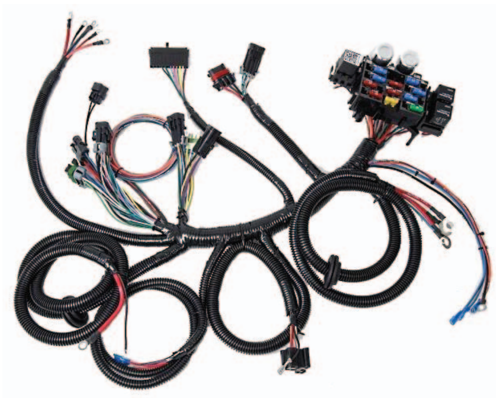
Main fuse panel Harness
