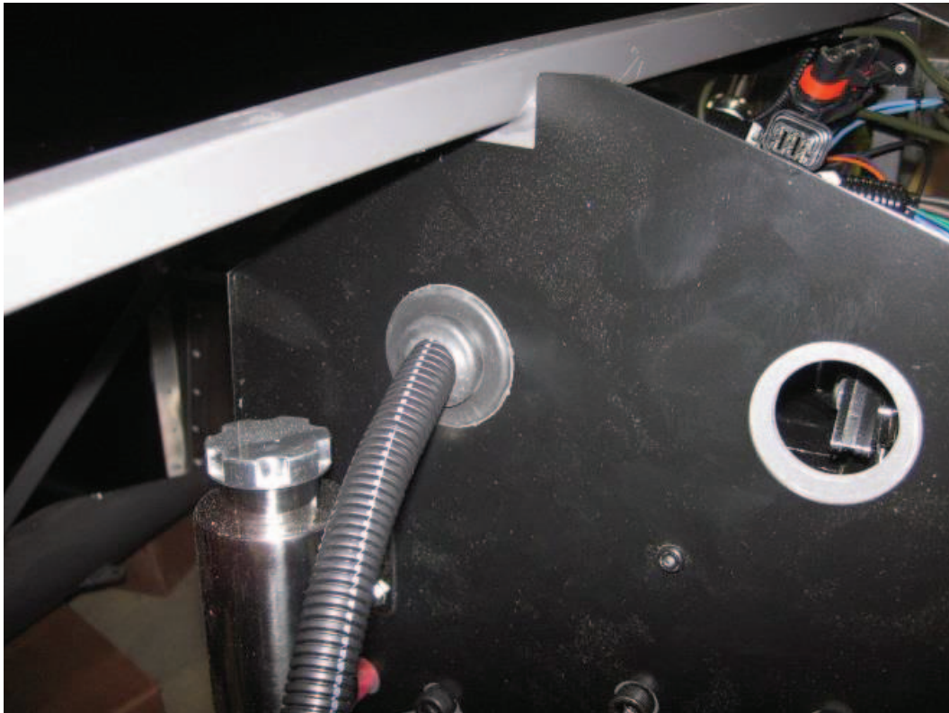
Pass the entire front harness connector through the hole and insert the grommet into the hole in the plate.
