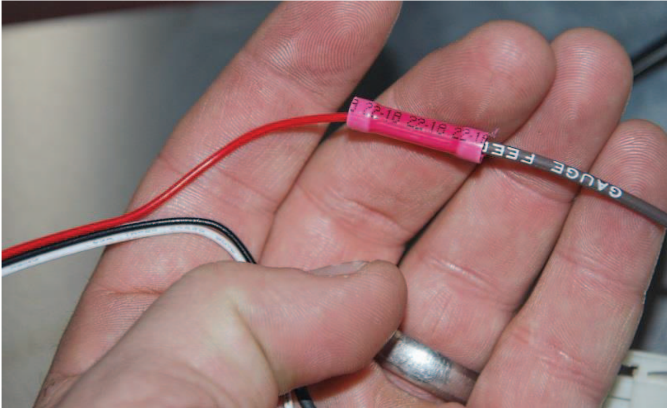
Connect the red power distribution wire to the brown gauge feed wire.
