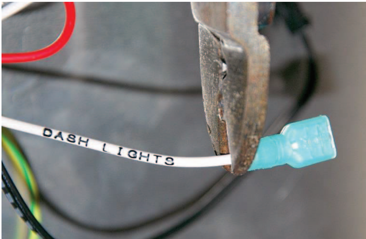
Cut the female connector off the end of the white dash lights wire.
