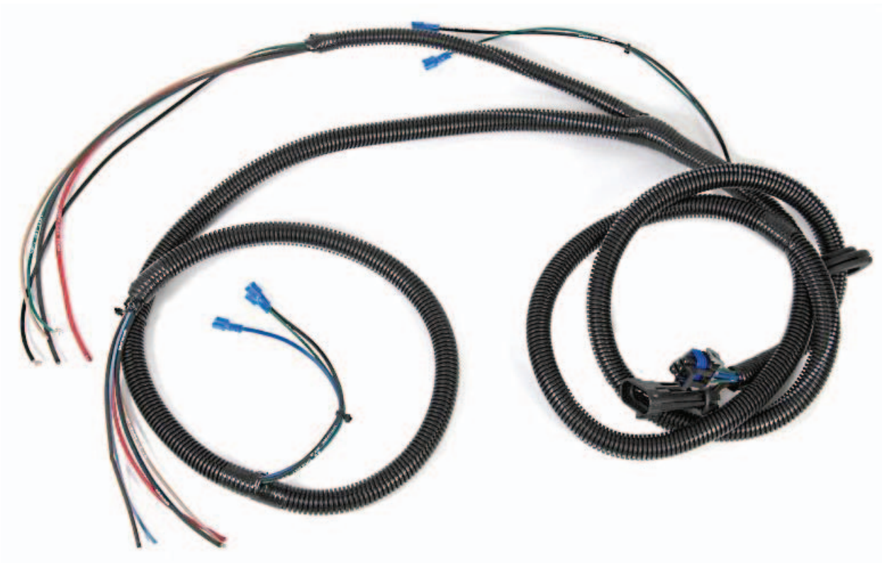
Front Harness
