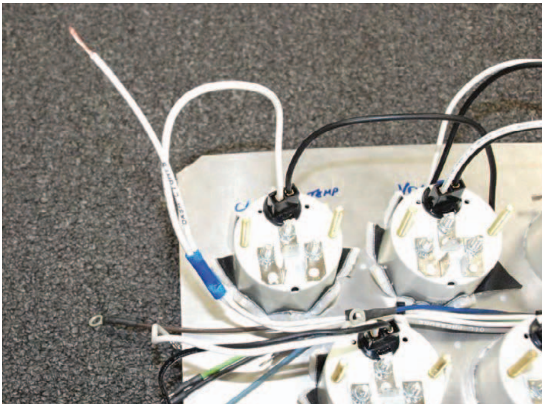
Connect the twisted wire to the white gauge light power wire.
